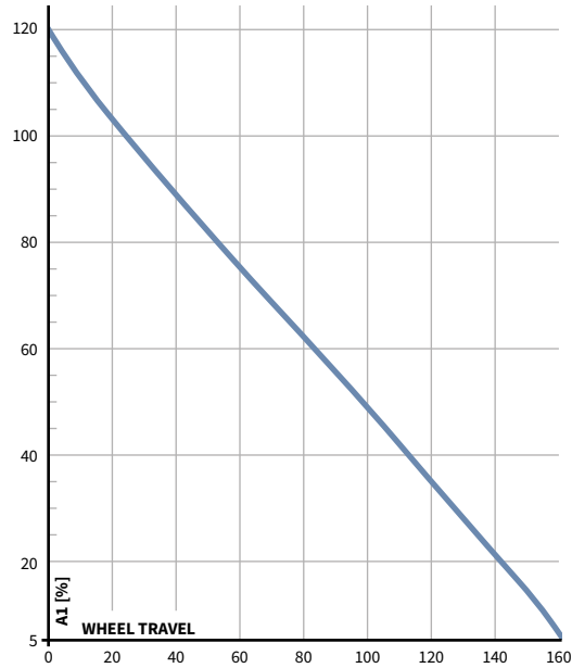
ANTI-SQUAT (36/28)
