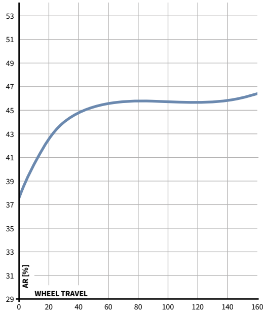
ANTI-RISE
