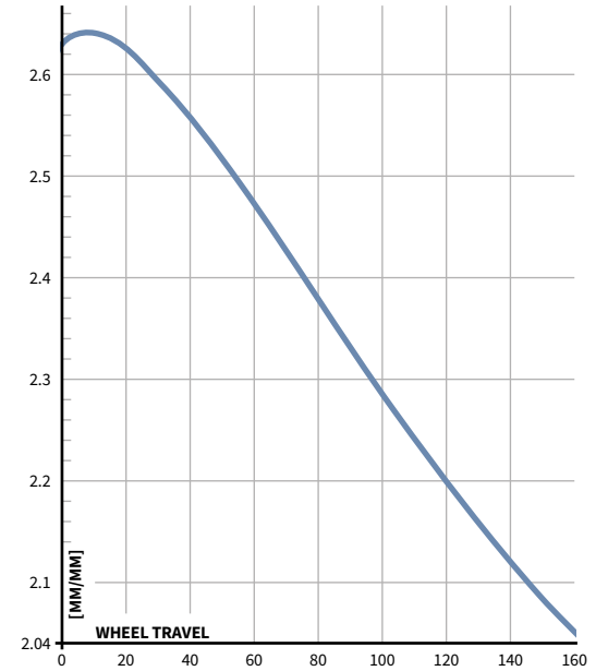
LEVERAGE RATIO
