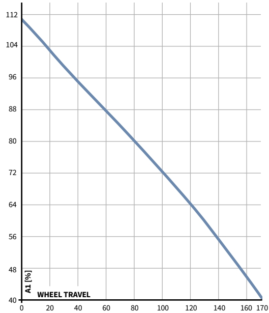
ANTI-SQUAT (34/24)
