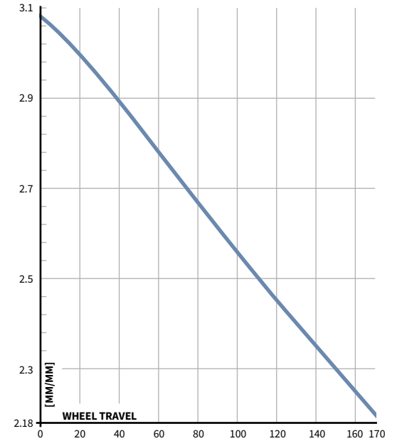
LEVERAGE RATIO
