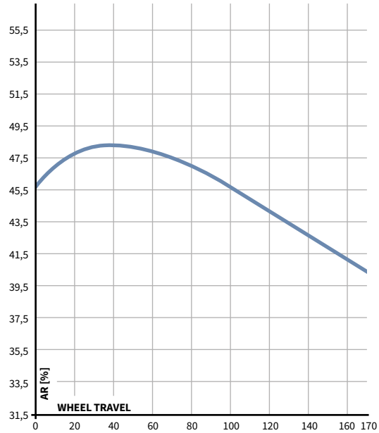
ANTI-RISE
